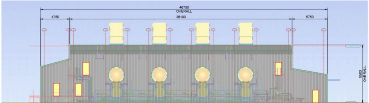
EXISTING ELEVATION - GRIDLINE 7 LOOKING WEST SCALE 1:200
