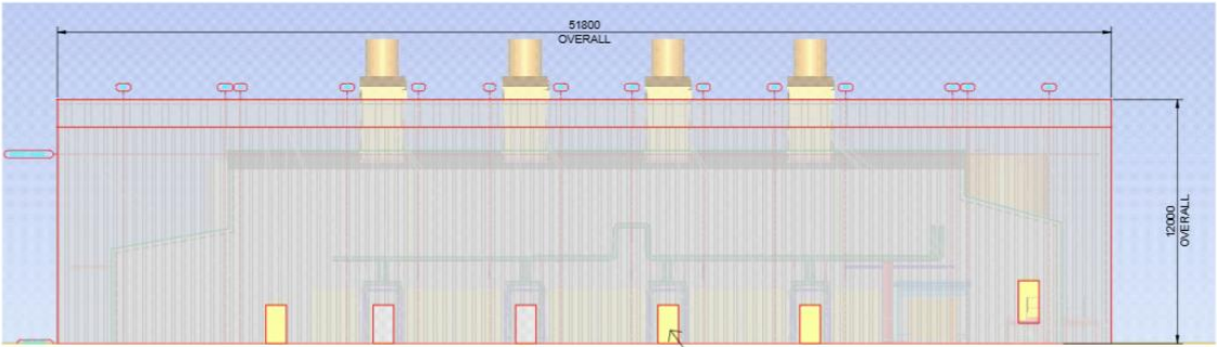
PROPOSED ELEVATION - GRIDLINE 1 LOOKING EAST SCALE 1:200
