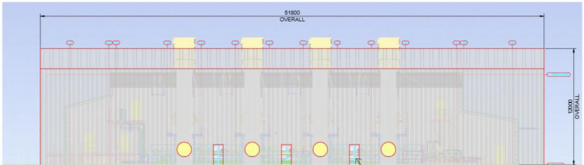
PROPOSED ELEVATION - GRIDLINE 7 LOOKING WEST
